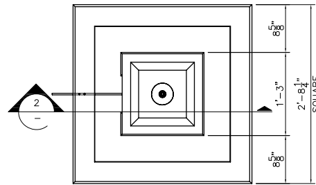
1 PLAN VIEW SCALE: 1/2"=1'
