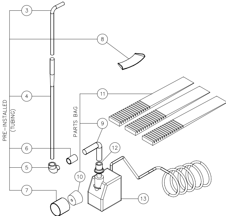
2 SECTION
