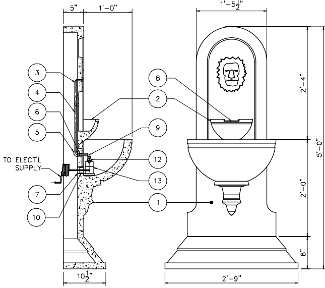
2 SECTION
