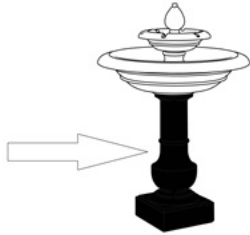
FT-299F (97 lbs) 11.5"L x 11.5"W x 25.75"H
